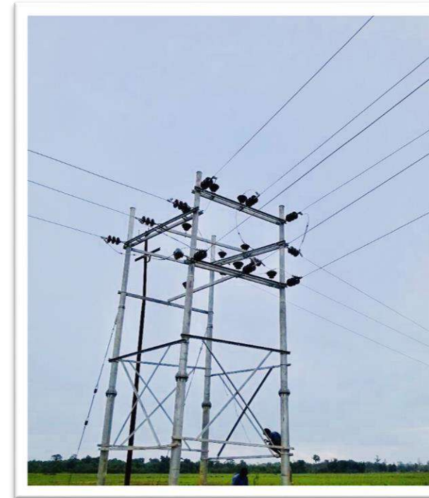
Overhead Line
